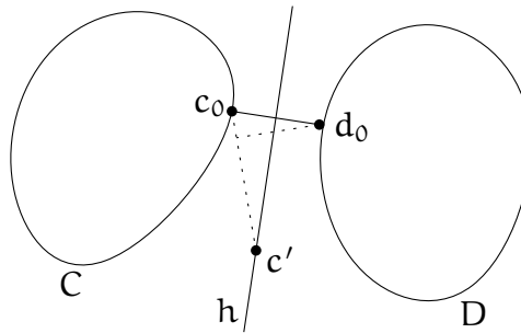
Figure 4.2: The hyperplane h strictly separates the compact convex sets C and D .
