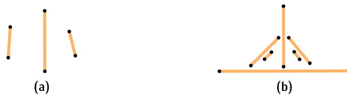
Figure 8.7: Sets of disjoint line segments that do not allow certain polygons.
