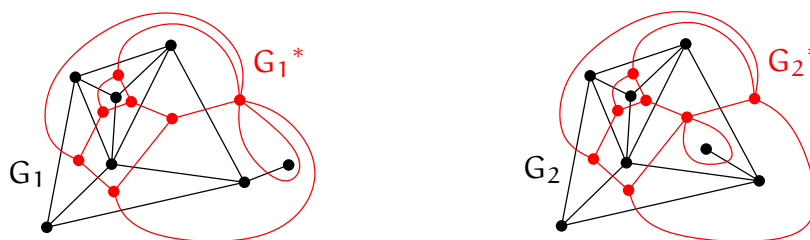
Figure 2.5: Two plane drawings G_1 and G_2 of the same abstract planar graph and their duals G_1^* and G_2^* with G_1^* \not\cong G_2^* . (To see this, for instance, count the number of vertices of degree greater than three.)
