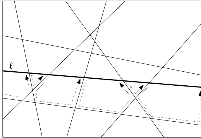
Figure 9.2: Incremental construction: Insertion of a line \ell . (Only part of the arrangement is shown in order to increase readability.)
