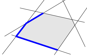
Figure 9.3: Left-bounding edges (blue and bold) of a cell.
