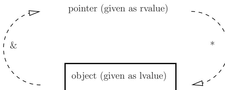
Figure 10: The address operator (left) and its inverse, the dereference operator (right)
